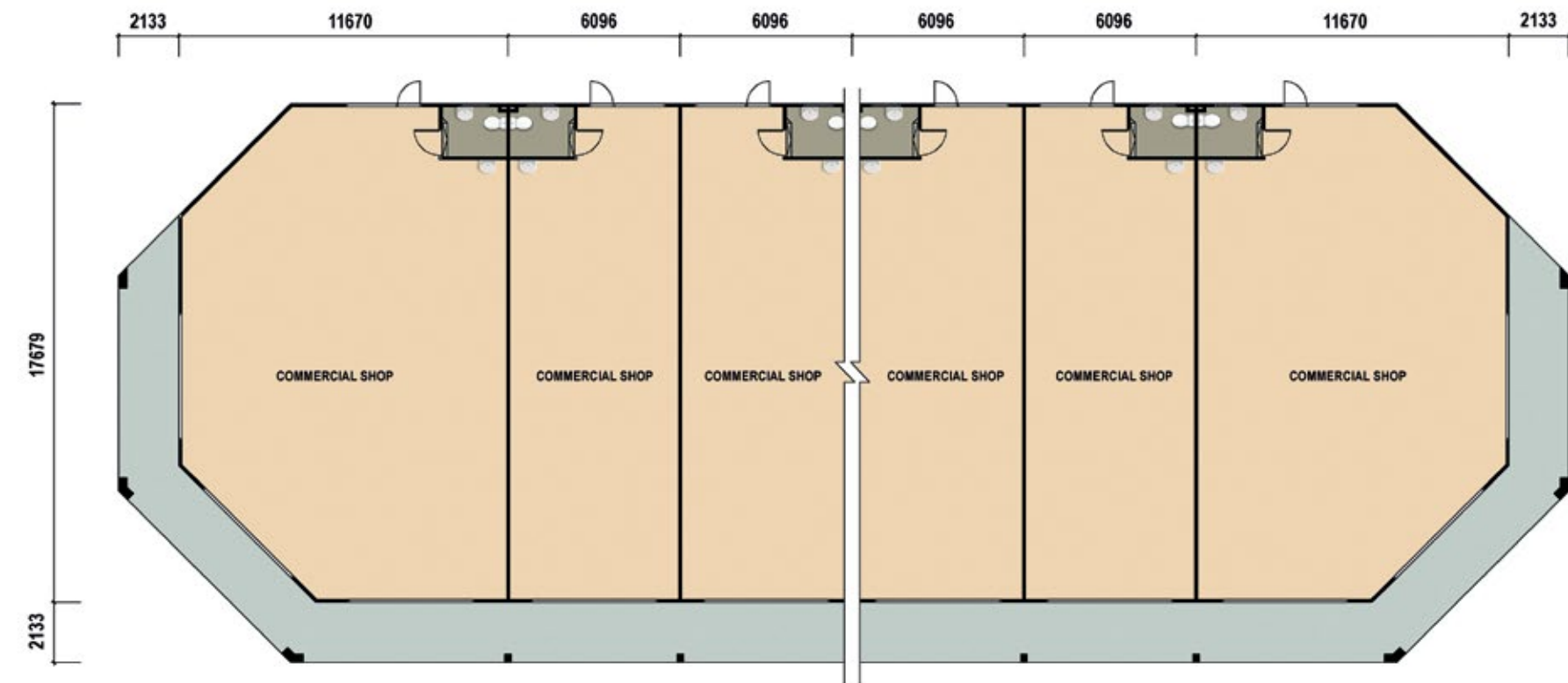
1-Storey Commercial Shops Lot Size: 20' x 65' Built-Up Area: 1,160 sq ft
